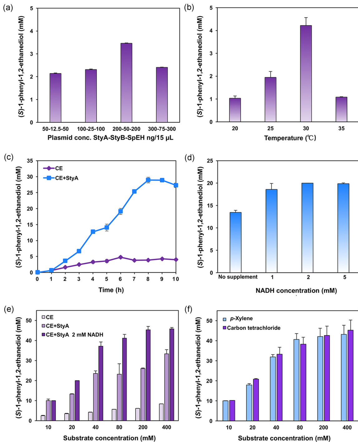
FIGURE 4 Optimization of (S)-1-phenyl-1,2-ethanediol production in the CFPS/emulsion system. (a) Optimization of plasmid concentration. Other conditions: substrate = 10 mM, reaction time = 10 hr, reaction temperature = 30 ^{\circ} C. (b) Optimization of reaction temperature. Other conditions: substrate = 10 mM, reaction time = 10 hr, plasmid (StyA–StyB–SpEH) concentration = 200–50–200 ng/15 \mu L. (c) Time courses of (S)-1-phenyl-1,2-ethanediol production with 40 mM styrene. (d) Effect of the additional supplement of NADH on (S)-1-phenyl-1,2-ethanediol formation with 20 mM styrene. (e) Production of (S)-1-phenyl-1,2-ethanediol with different styrene concentrations in three reaction systems. (f) Production of (S)-1-phenyl-1,2-ethanediol with different styrene concentrations in two CFPS/emulsion systems ( p -xylene and carbon tetrachloride). Three independent CFPS reactions were performed for each condition, and one standard deviation is shown. CE, cell extract without overexpressed StyA; CE + StyA, StyA-enriched cell extract; CE + StyA 2 mM NADH, StyA-enriched cell extract plus 2 mM NADH in the reaction; CFPS, cell-free protein synthesis; SpEH, epoxide hydrolase [Color figure can be viewed at wileyonlinelibrary.com ]
