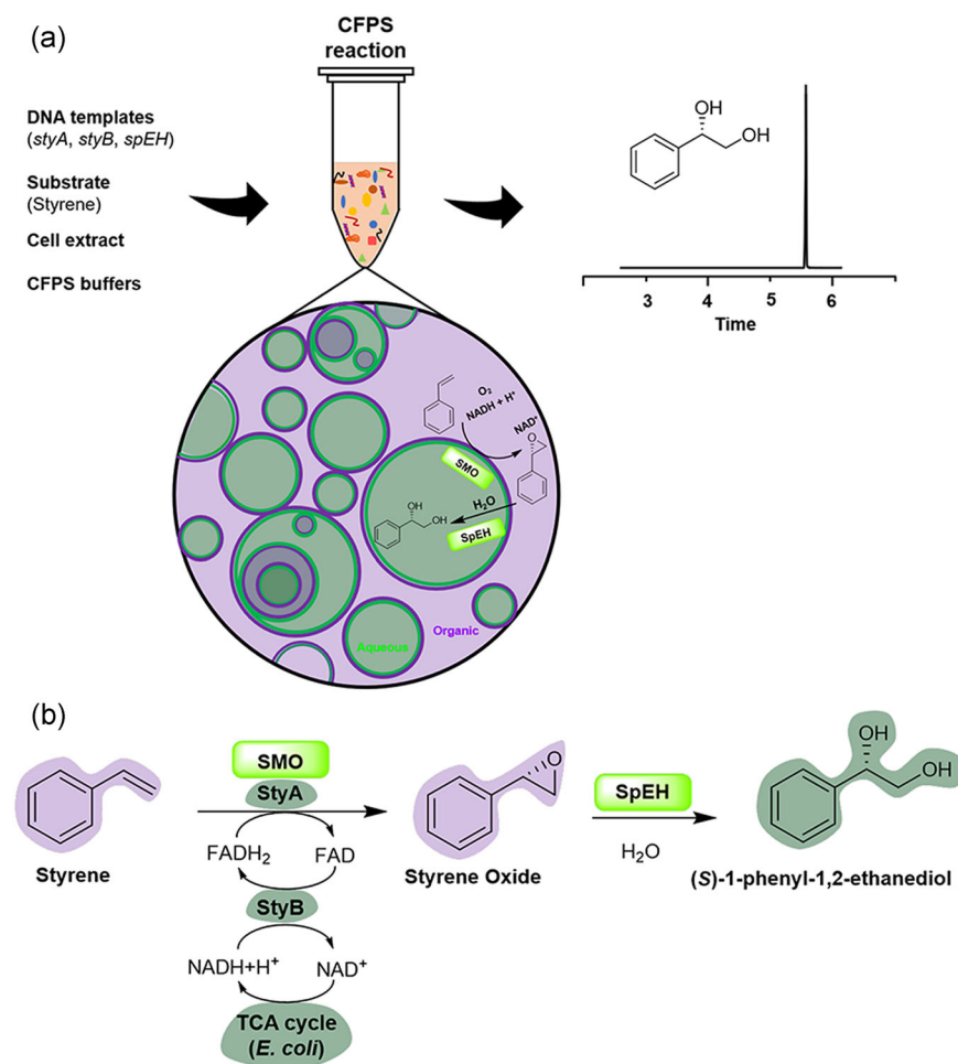
FIGURE 1 (a) Schematic diagram of one-pot cascade biotransformation from styrene to ( S )-1-phenyl-1,2-ethanediol in a CFPS/emulsion system. (b) Overall two-step enzymatic cascade reactions. CFPS, cell-free protein synthesis; SMO, styrene monooxygenase; SpEH, epoxide hydrolase; TCA cycle, tricarboxylic acid cycle [Color figure can be viewed at wileyonlinelibrary.com ]
