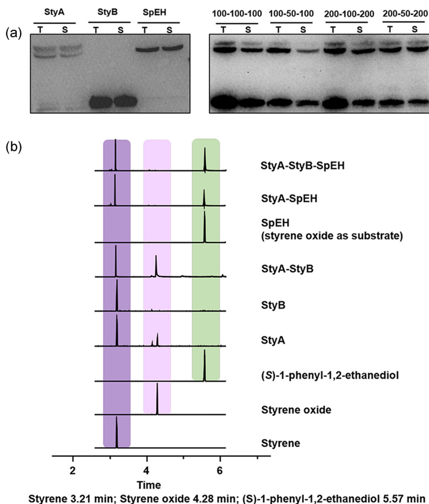
FIGURE 3 (a) Western-blot analysis of individual expression (left) and coexpression (right) of StyA (46.3 kDa), StyB (18.4 kDa), and SpEH (42.9 kDa) labeled with the anti-His antibody. Numbers on the top of the right panel indicate three plasmid concentrations (StyA–StyB–SpEH) per 15 μl CFPS reaction. Note that the below band of StyA (left) is a truncated protein. (b) GC–MS detection of substrate (styrene), intermediate (styrene oxide), and product ((S)-1-phenyl-1,2-ethanediol). The concentrations of styrene and styrene oxide were 10 mM when they were used as substrates in the reaction. Three independent reactions were performed for each condition, and an example trace is shown. CFPS, cell-free protein synthesis; GC–MS, gas chromatography–mass spectrometry; S, soluble protein; SpEH, epoxide hydrolase; T, total protein [Color figure can be viewed at wileyonlinelibrary.com ]
