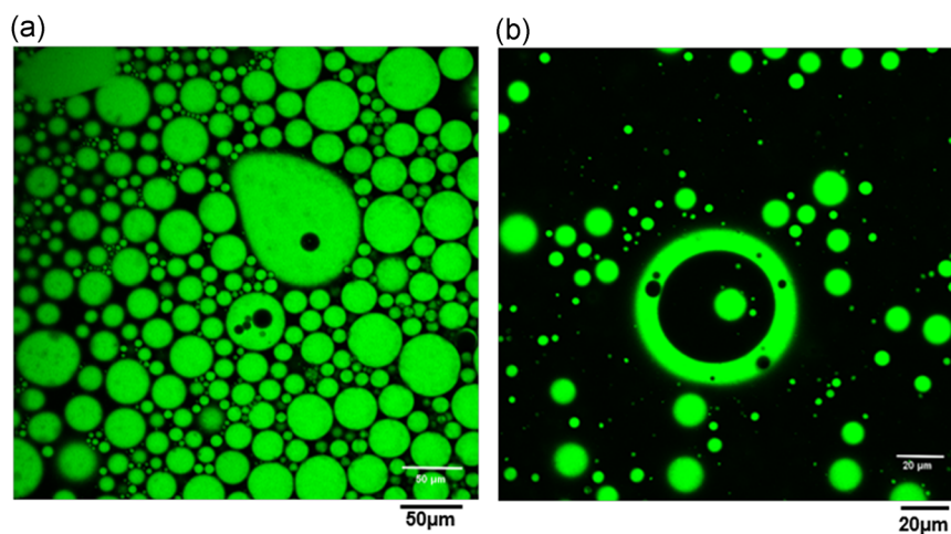
FIGURE 2 Cell-free synthesis of sfGFP in the CFPS/emulsion system and the single-/multi-compartmentalized structures of the emulsion detected by confocal laser scanning microscopy (A: \times 20 and B: \times 40 ). CFPS, cell-free protein synthesis; sfGFP, super-folder green fluorescent protein [Color figure can be viewed at wileyonlinelibrary.com ]
