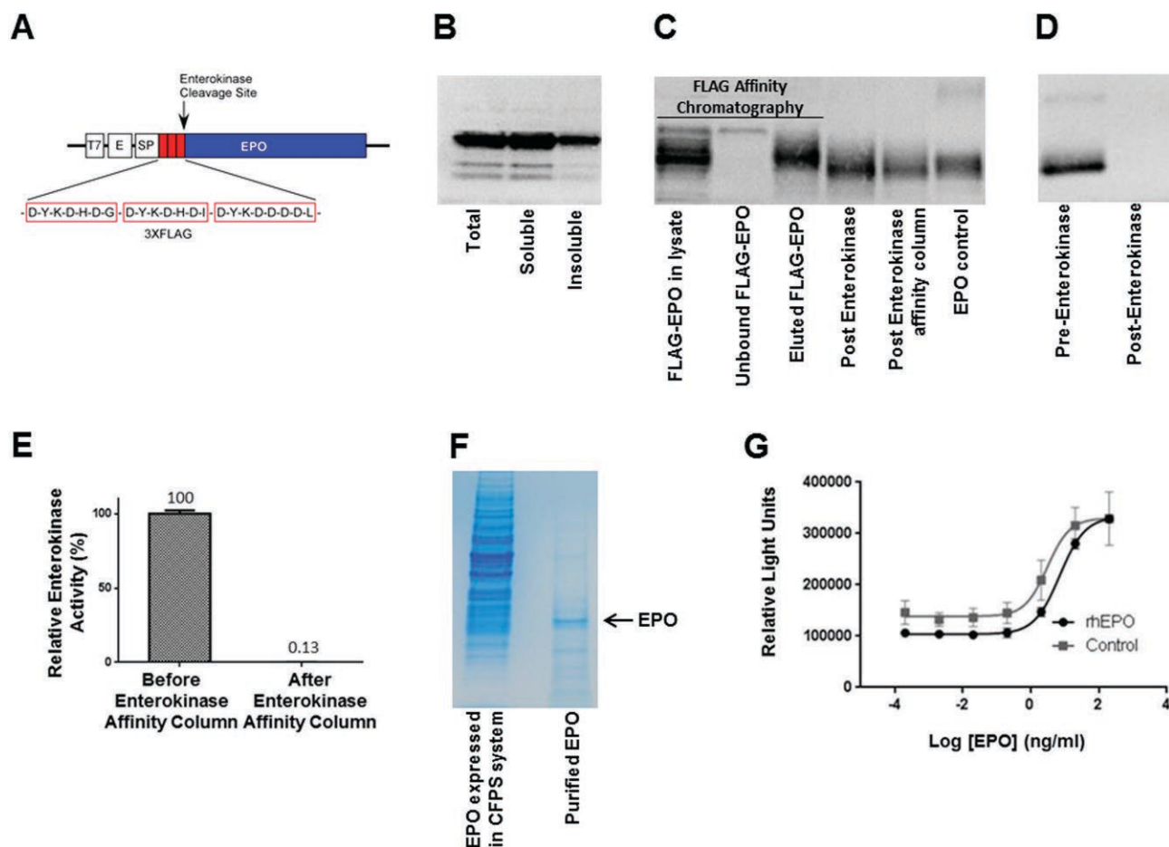
Figure 3. Expression and purification of recombinant human EPO using the fluidics system. (A) Schematic diagram of the construct used for cell-free expression of rhEPO in the yeast CECF protein synthesis system. The PCR template for rhEPO contains a T7 promoter (T7), translational enhancer (E), signal peptide (SP), and three FLAG epitopes, with an Enterokinase cleavage site upstream of the mature coding sequence. (B) Western blot analysis of rhEPO expression in a yeast cell-free protein synthesis system at 22°C. The majority of rhEPO expressed in the yeast CFPS system is present in the soluble fraction. (C) Western blot analysis (anti-EPO) of FLAG-rhEPO expressed in a yeast cell-free protein synthesis system during the various steps of protein purification. (D) Western blot analysis (anti-FLAG) of EPO sample before and after Enterokinase treatment for FLAG-tag removal. (E) The efficiency of the Enterokinase capture and removal step assessed using a fluorogenic substrate-based enzymatic assay; upon enzyme cleavage, this substrate generates a rhodamine fluorophore that is detected at excitation/emission = 490/520 nm. (F) Coomassie blue staining of protein samples before and after FLAG-affinity chromatography. (G) Biological activity of rhEPO synthesized in a PDMS-based reactor hosting a yeast CFPS system under continuous exchange format and purified as described in Fig. 1B. Protein biological activity was assessed using a standard human TF-1 cell-based proliferation assay. Shown are representative results from two biological replicates at multiple rhEPO protein concentrations. Data represent the mean ± SD of luminescence relative light units produced in the biological experiments.
