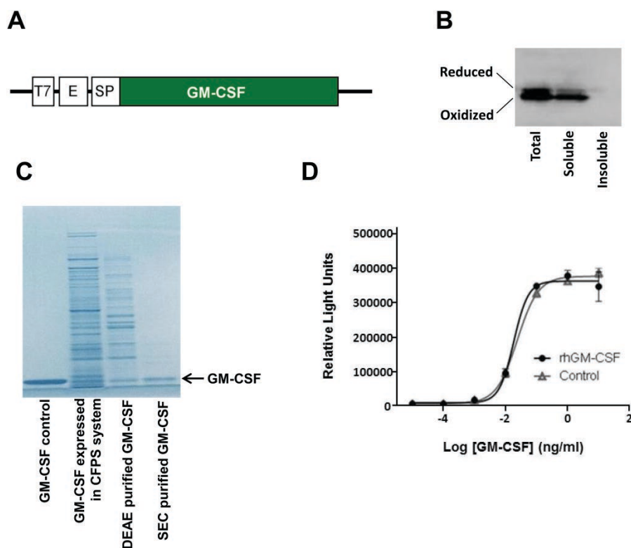
Figure 4. Expression and purification of recombinant human GM-CSF using the fluidics system. (A) Schematic diagram of the construct used for cell-free expression of rhGM-CSF in the bacterial cell-free protein synthesis system. The plasmid template for rhGM-CSF contains a T7 promoter (T7), translational enhancer (E), and signal peptide (SP) upstream of the mature coding sequence. (B) Western blot analysis of cell-free expressed rhGM-CSF in a bacterial lysate. CFPS reaction was performed in the presence of nonionic detergent Brij-35 (0.1%), IAM and DsbC at 30°C. (C) Purification of rhGM-CSF expressed in bacterial CFPS system. Coomassie blue staining of protein fractions during the various steps of the purification process. Commercial human GM-CSF was used as a control. (D) Biological activity of rhGM-CSF synthesized in a PDMS-based reactor hosting a bacterial CFPS system under batch format and purified as described in Fig. 1C. Protein biological activity was assessed using a standard human TF-1 cell-based proliferation assay. Shown are representative results from two biological replicates at multiple rhGM-CSF protein concentrations. Data represent the mean \pm SD of luminescence relative light units produced in the biological experiments.
