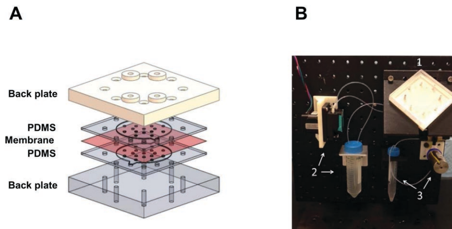
Figure 2. Protein synthesis reactor. (A) A computer-aided design model of the protein synthesis reactor for hosting cell free protein synthesis under continuous exchange format. Dotted features are “stand-off” supports to maintain channel volume by constricting dialysis membrane motion. (B) Protein synthesis reactor, feeder and sample loading modules. (1) Protein synthesis reactor. The reactor consists of a 2 mL polydimethylsiloxane (PDMS) chamber divided into the reaction and feeding chambers (1 mL, each) by a 3.5 kDa dialysis membrane. Molded PDMS chambers were produced from a stereo-lithographic printed mold. (2) Peristaltic pump and storage vial for feeder solution loading to the feeding chamber of the reactor and recirculation. (3) Diaphragm and vial for reagents loading to the reactor chamber and sample recovery.
