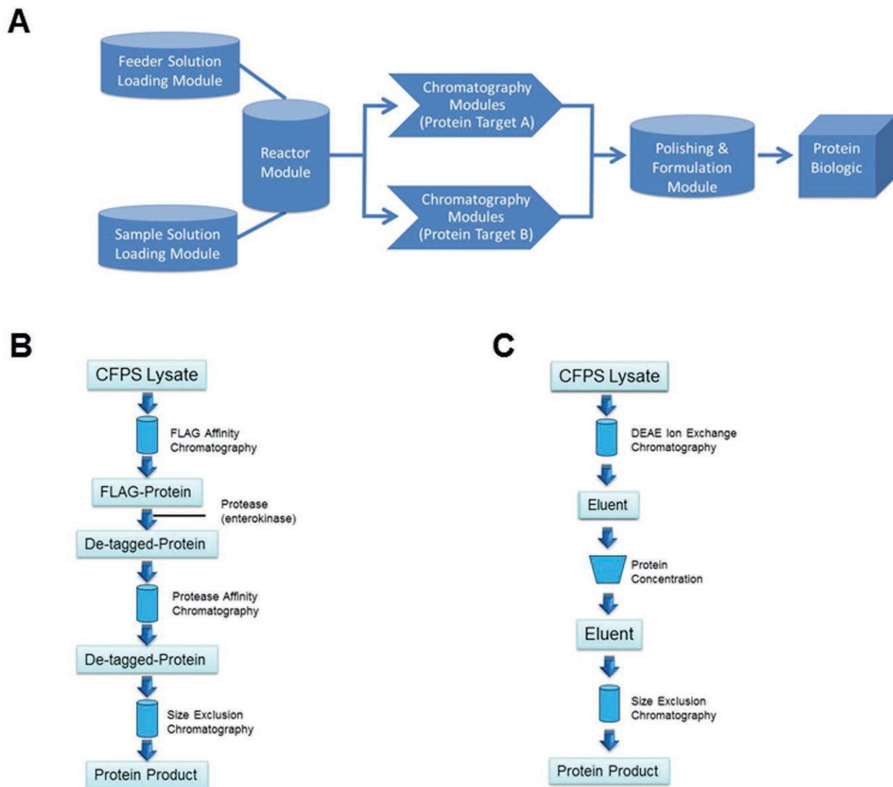
Figure 1. A schematic diagram of the fluidic process for cell-free production of protein biologics. (A). The fluidic process consists of: (i) Reagents (feeder and sample solutions) loading to the reactor system; (ii) Combined transcription/translation step taking place in a reactor module under continuous exchange or batch format; (iii) Protein purification steps for separation of the target proteins from the lysate mixtures using a variety of chromatography matrices depending on protein target modalities; and (iv) Protein polishing and formulation step, typically through the use of a size exclusion chromatography matrix. (B). Schematic representation of the purification process for recovery of rhEPO from a yeast cell-free protein synthesis system. This method incorporates FLAG-tag-based affinity chromatography for protein recovery from the cell-free system with subsequent removal of the affinity tag for recovery of the intended size protein target. (C). Process diagram for purification of rhGM-CSF from a bacterial cell-free protein synthesis system via the use of anion-exchange chromatography in combination with size exclusion chromatography.
