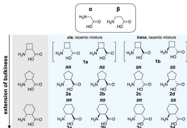
Fig. 1 Expanding the chemical substrate scope of ribosome-mediated polymerization to cyclic \beta -amino acid (c \beta AA) substrates. We explore the substrate specificity of the natural translation machinery for c \beta AA substrates using flexizyme-catalyzed acylation and ribosome-mediated incorporation. Ten non-canonical c \beta AAs comprising a variety of bulky cyclic structures are investigated.
